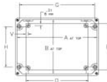
Top View with Cover Removed
