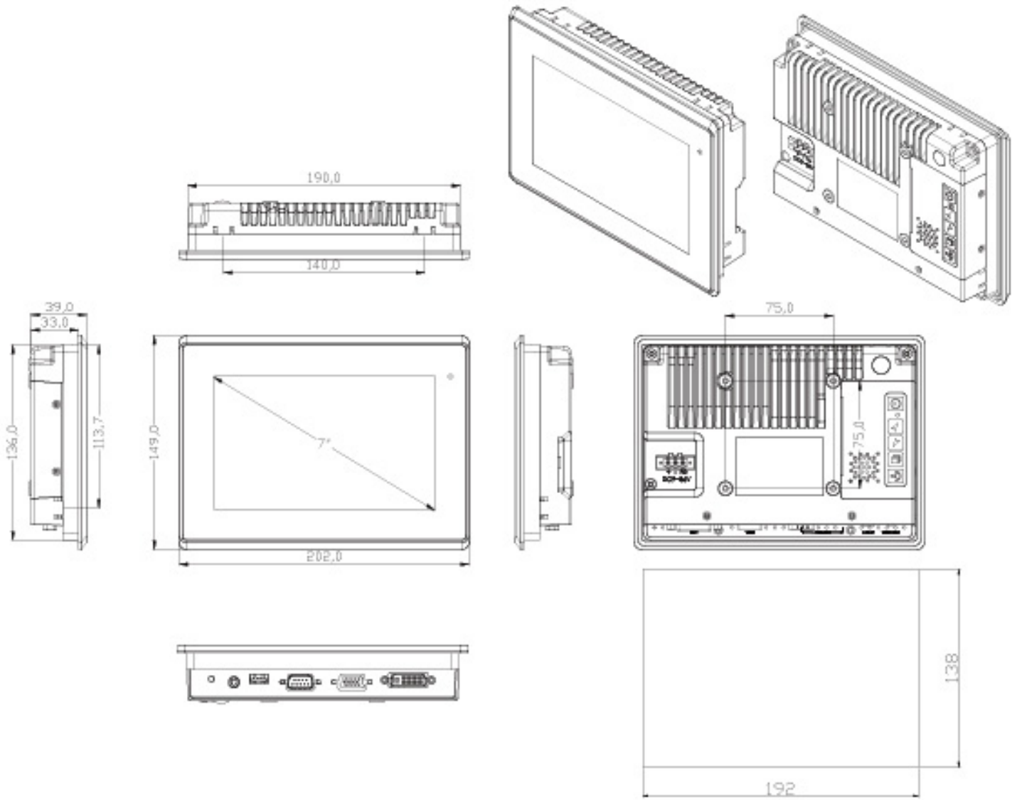
Mounting Hole Size
