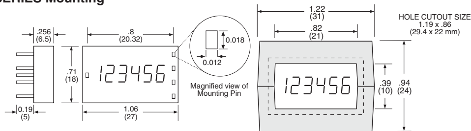
MINI-KAL1 SERIES with KALPM1 panel adaptor clips into panel .050 to .125 thick
